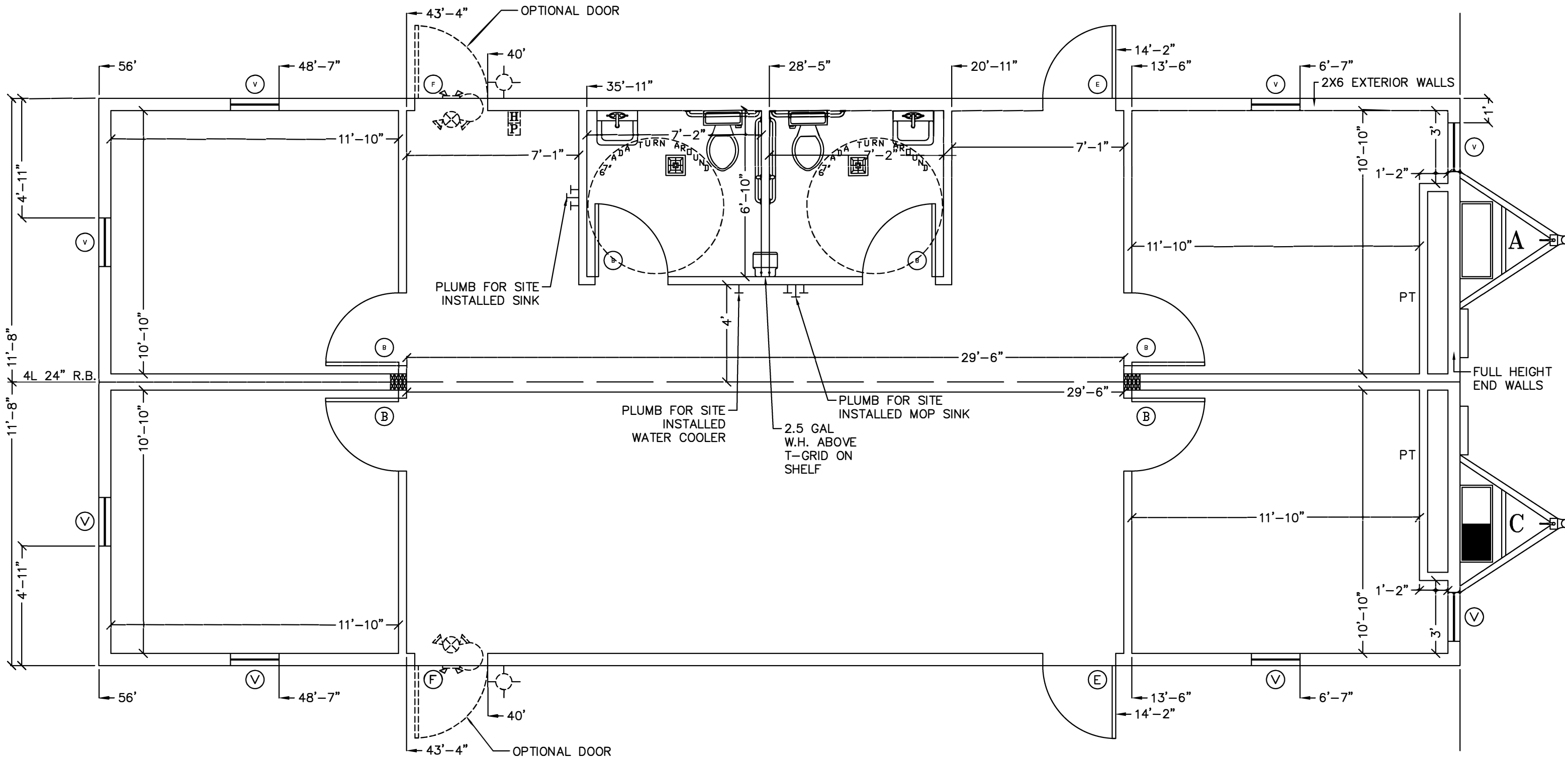
PLEX Double Wide 24 x 56 Floor Plan
