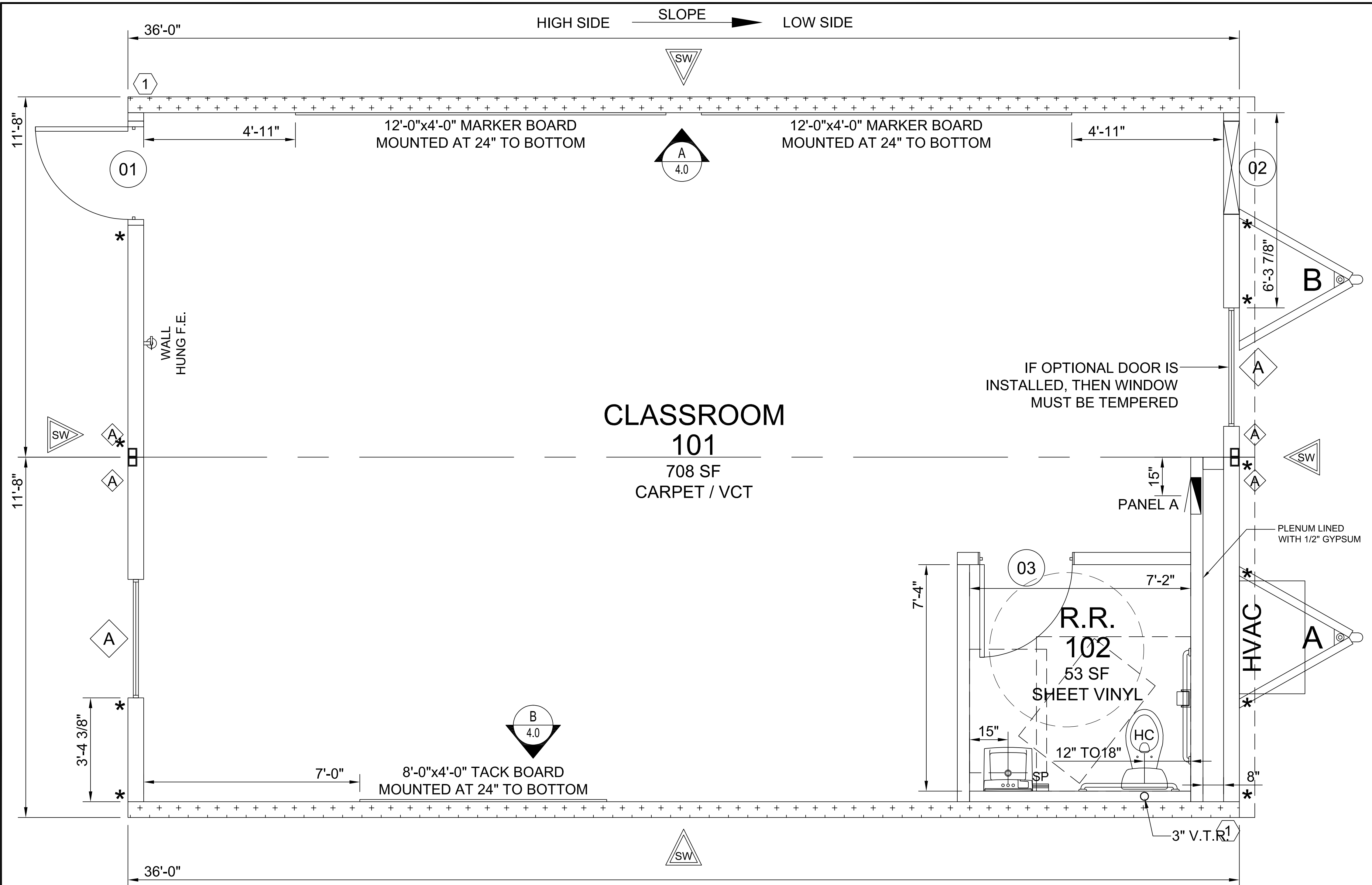
1 FLOOR PLAN 1/4"=1'-0" SQUARE FOOTAGE - 834 S.F. OCCUPANCY LOAD = 35
