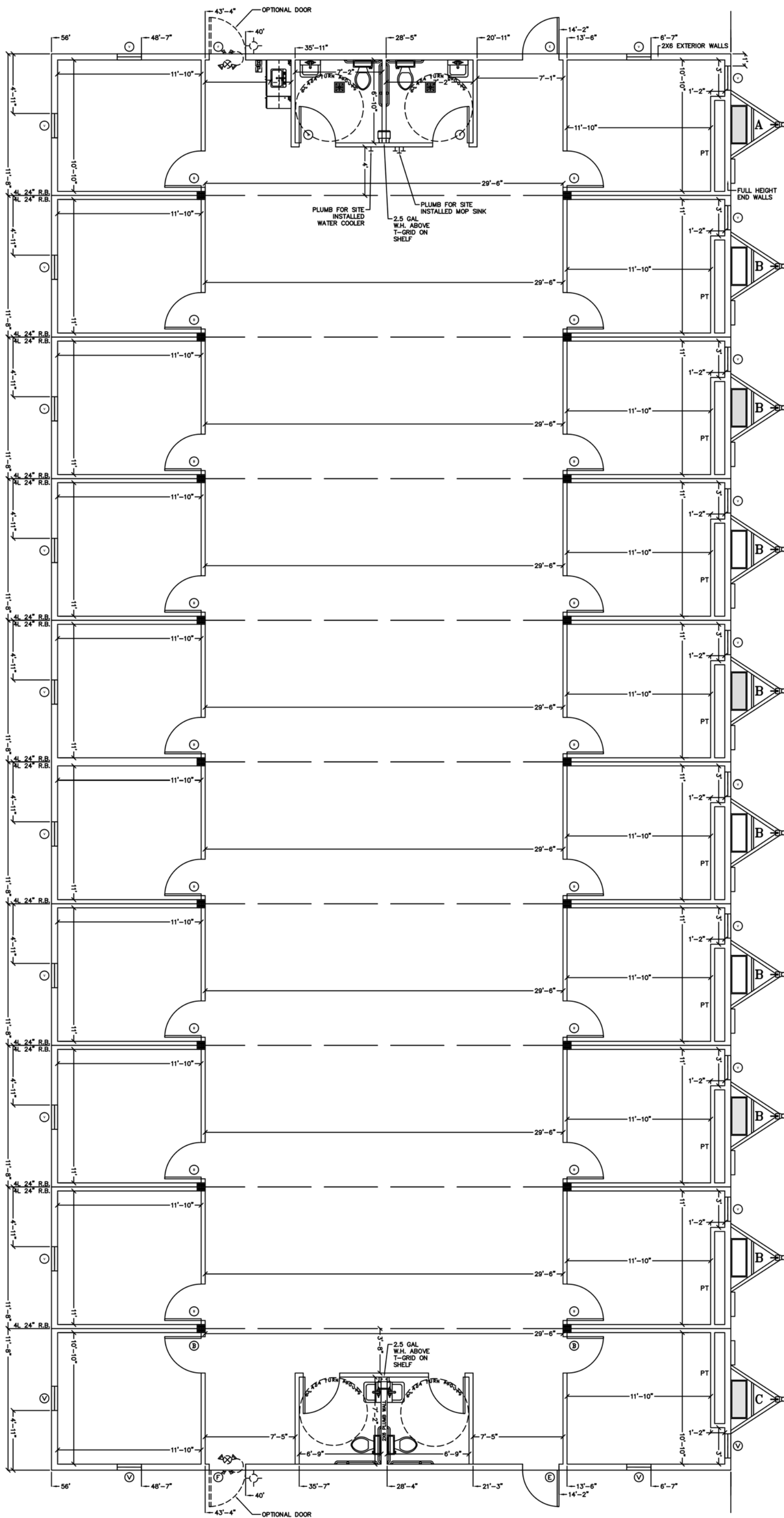
10 PLEX Wide 120 x 56 Floor Plan
