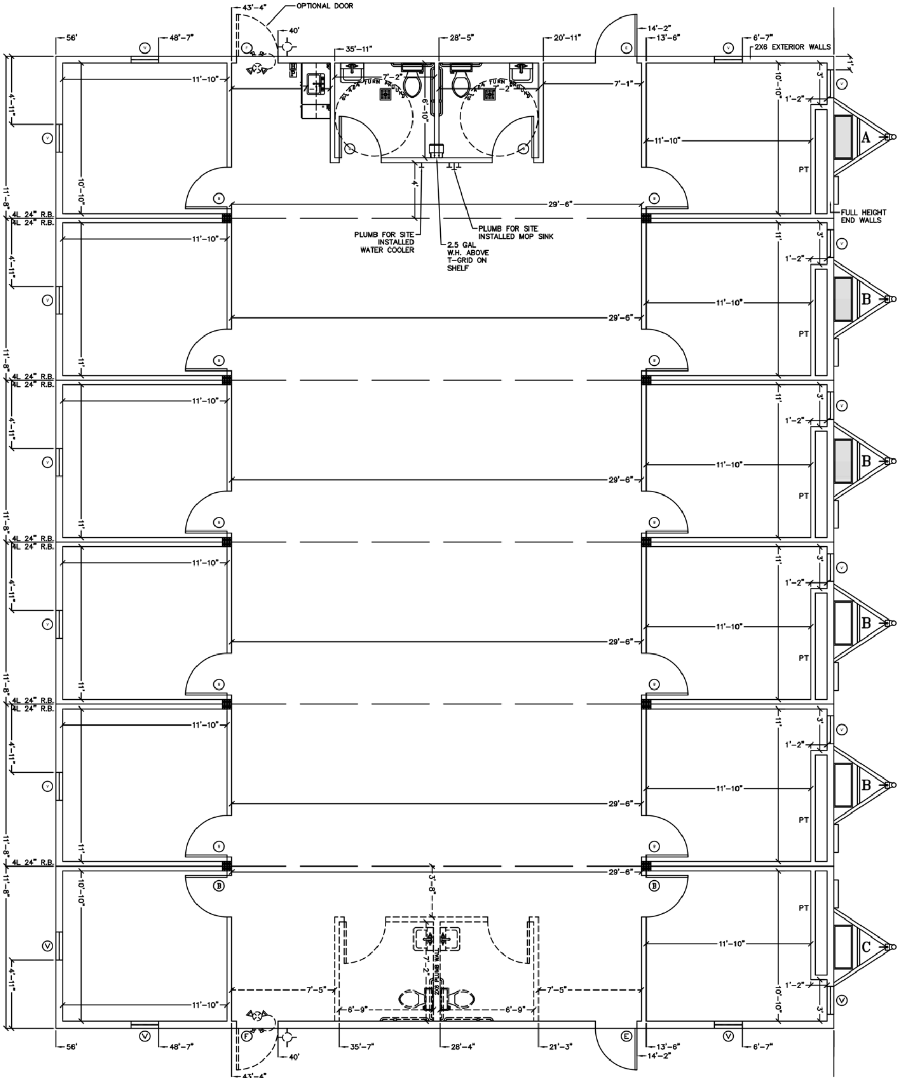
6 PLEX Wide 72 x 56 Floor Plan
