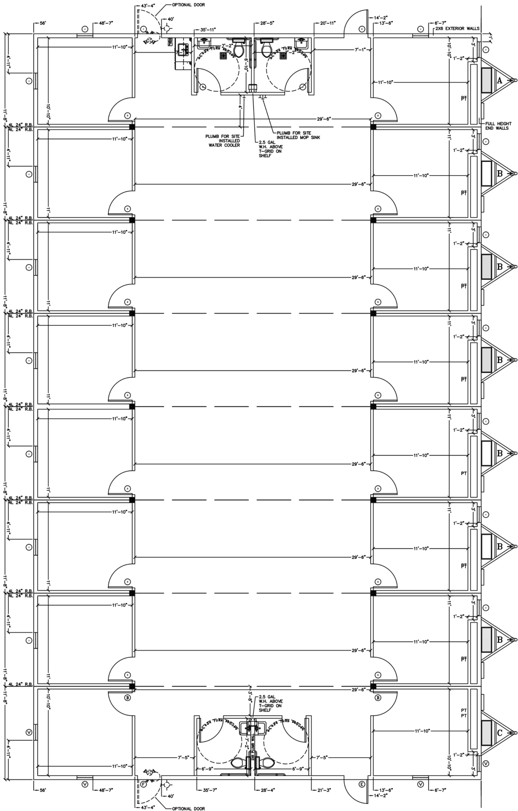
9 PLEX Wide 108 x 56 Floor Plan
