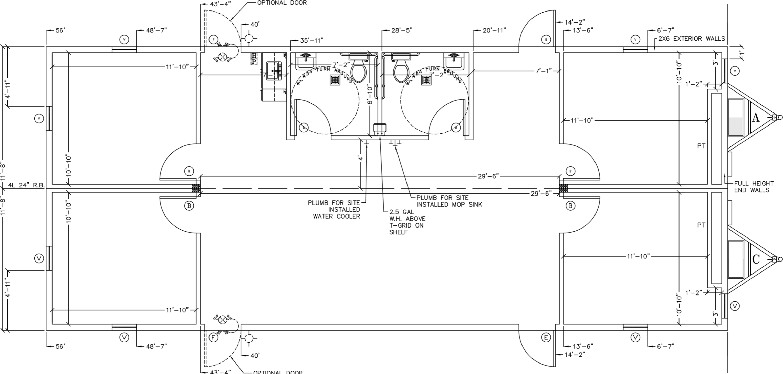
PLEX Double Wide 24 x 56 Floor Plan
